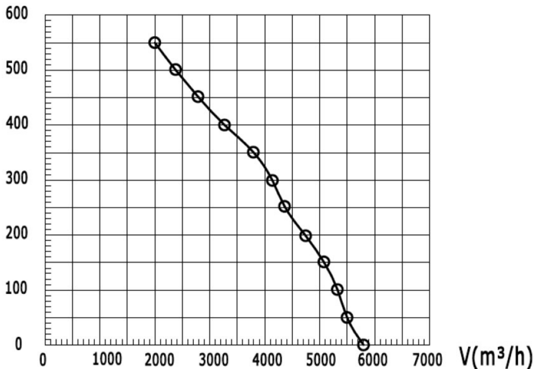
Airflow curves
